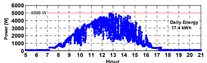
Fig. 1: Output power of a PV arrays during a partially cloudy day.
