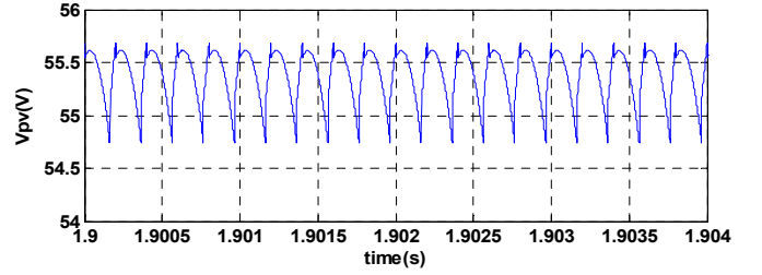
Fig. 10. PV voltage ripple at 1000 W/m² irradiance.
