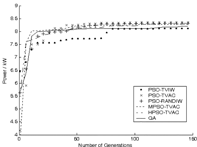
Fig. 3. Variation of optimum power with generations.
