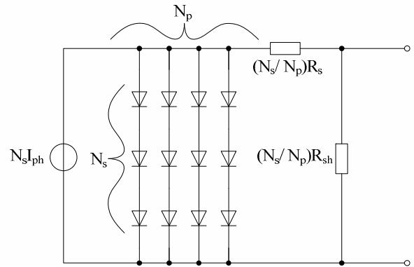
Fig. 4. Cells influence on PV solar module equivalent circuit components.
