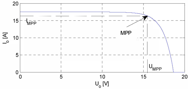
Fig. 2. Theoretical I-V characteristics of PV solar cell
