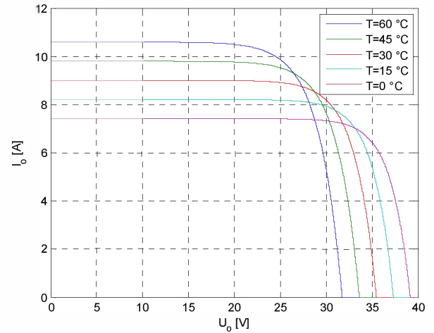
Fig. 9. Temperature I-V characteristics.
