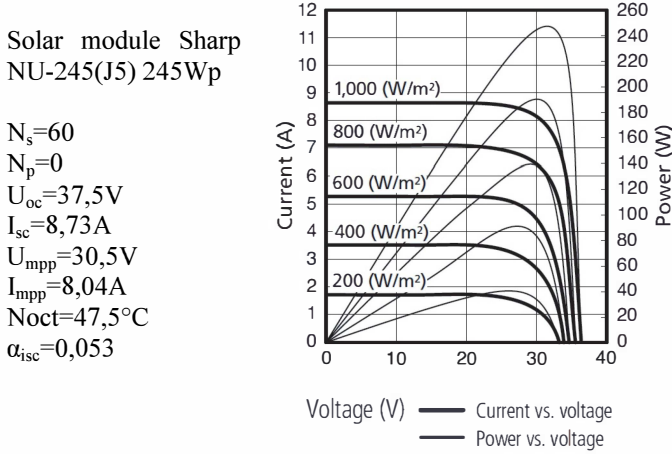
Fig. 5. Sharp NU-245(J5) 245Wp specifications and I-V characteristics.
