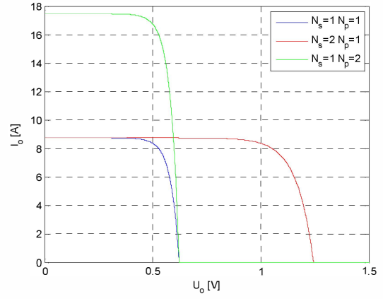
Fig. 3. Number of cells influence on output parameters.
