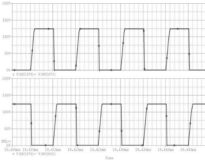
Figure 7. The voltage of the switches.
