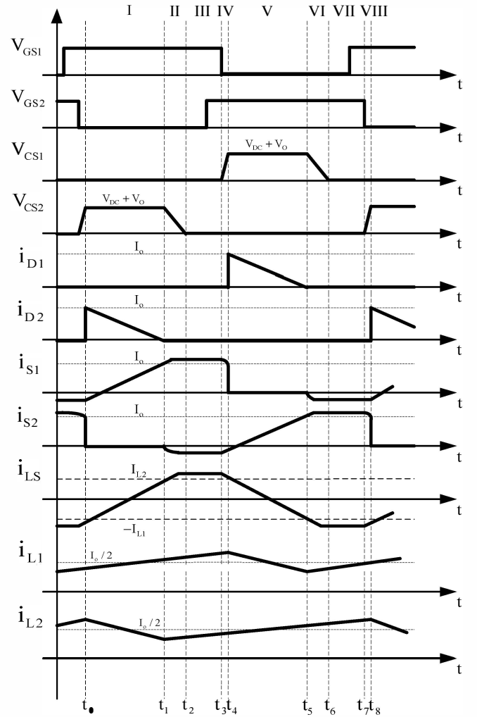
Figure 4. Theoretical waveforms.
