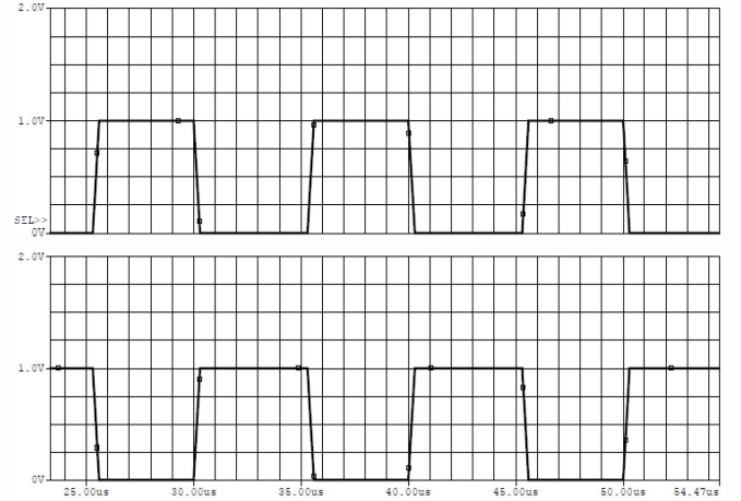
Figure 5. Gating signals of the switches.
