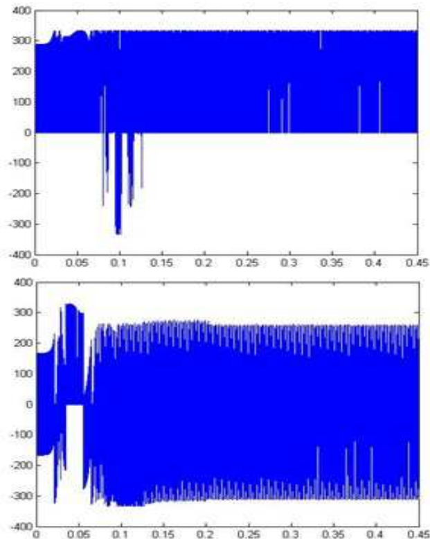
Fig.10. Transformed direct and quadrature axis stator voltages from three phase voltages
