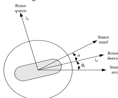
Fig.1. d-q model of Permanent magnet synchronous motor
