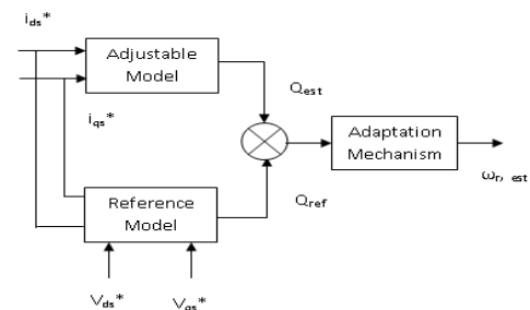
Fig.3. Functional block diagram of MRAS
