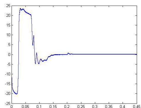
Fig.6. Direct axis stator current of PMSM drive
