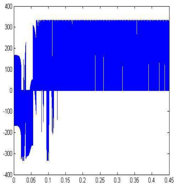
Fig.9. Quadrature axis stator voltage of PMSM drive
