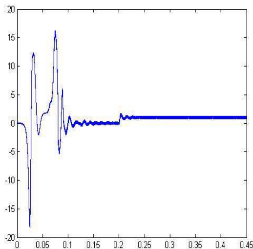
Fig.14. Electromagnetic torque of PMSM drive
