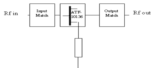
Figure 2 UWB LNA
