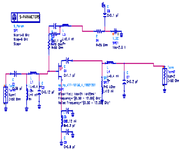
Figure 3 Schematic of the series UWB feedback LNA
