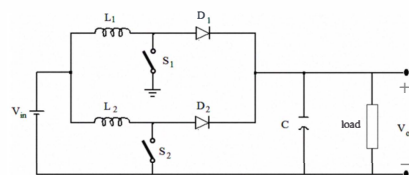
Fig. 2. The novel Boost converter
