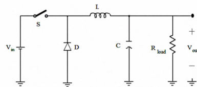
Fig. 8. The Conventional Buck Converter
