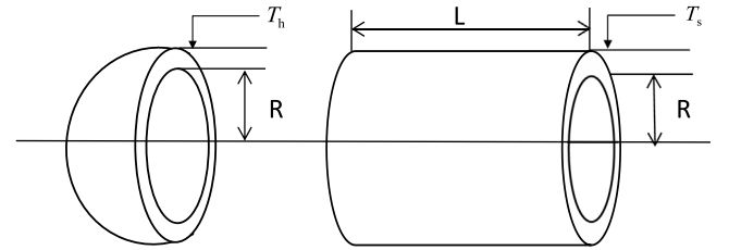
Fig. 14. Pressure vessel design – PVD.
