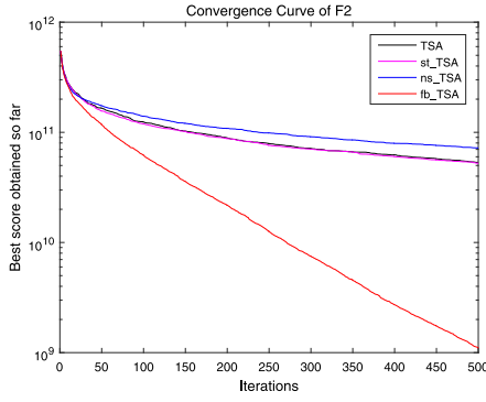
(a) f_2 , unimodal function
