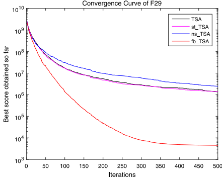
(e) f_{29} , composition function
