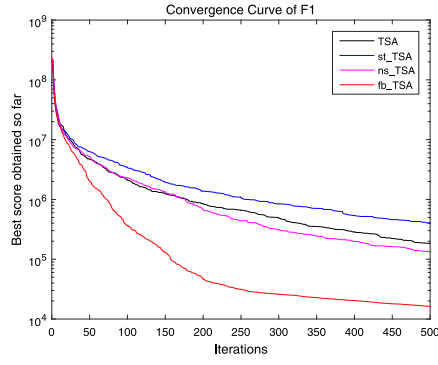
(a) f_1 , unimodal function
