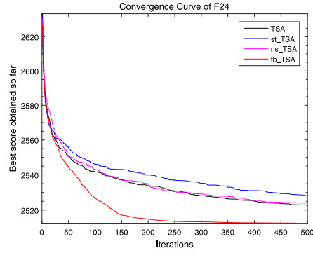
(e) f_{24} , composition function
