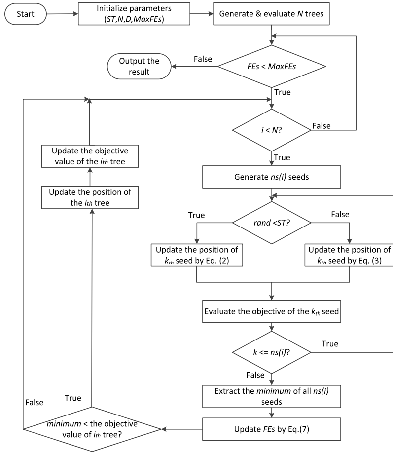
Fig. 1. Flow chart of the basic TSA.
