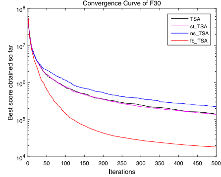
(f) f_{30} , composition function
