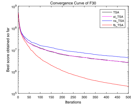
(f) f_{30} , composition function
