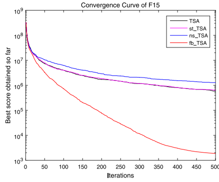
(c) f_{15} , multimodal function
