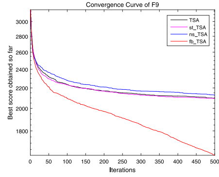
(b) f_9 , multimodal function
