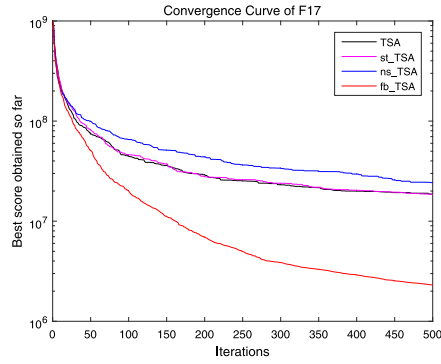
(c) f_{17} , hybrid function
