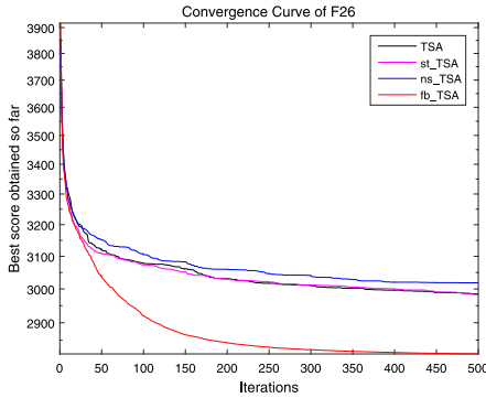
(e) f_{26} , composition function
