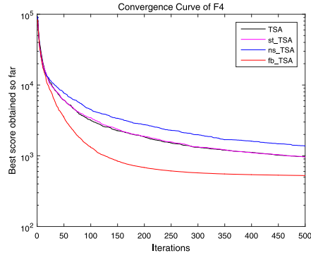
(a) f_4 , multimodal function
