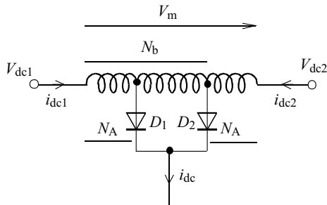
Fig. 5. Tapped inter-phase transformer circuit
