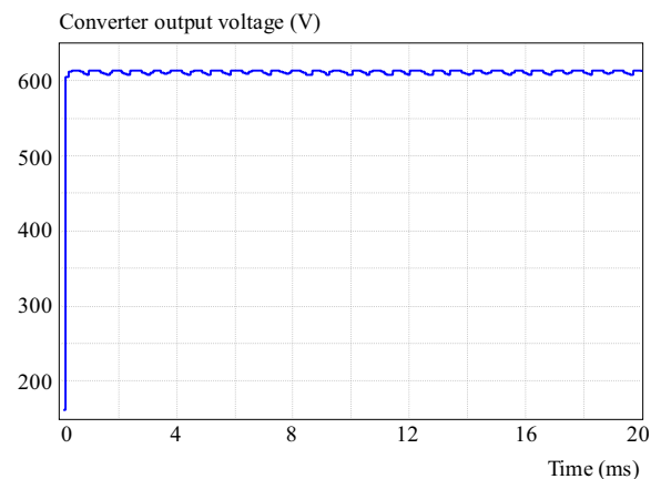
Fig. 9. 24-pulse ac-dc converter output voltage
