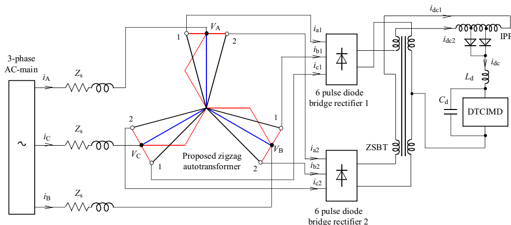
Fig. 3. Zigzag transformer configuration for 24-pulse ac-dc conversion
