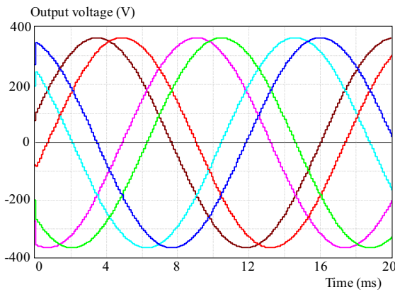
Fig. 6. Six-pulse autotransformer output voltage
