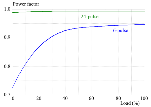
Fig. 12. Variation of power factor with load on DTCIMD in 6-pulse, 12-pulse and 24-pulse ac-dc converter
