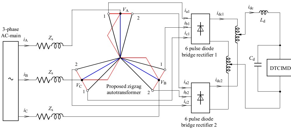
Fig. 1. Zigzag-autotransformer configuration for 12-pulse ac-dc conversion
