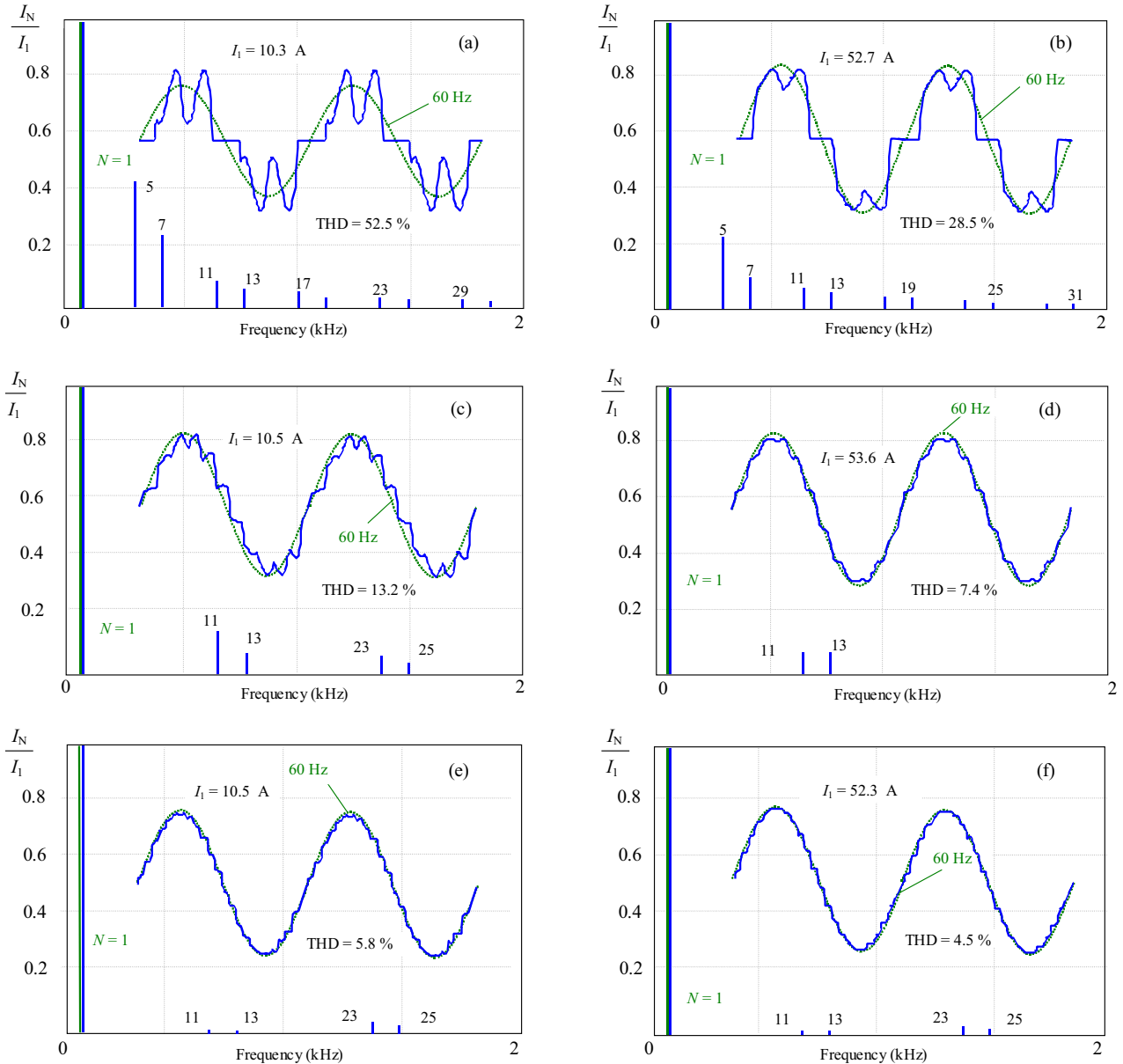
Fig. 10. Input current waveform of ac-dc converters and its harmonic spectrum at light load and full load at: (a),(b) – 6-pulse, (c),(d) – 12-pulse, and (e),(f) – 24-pulse
