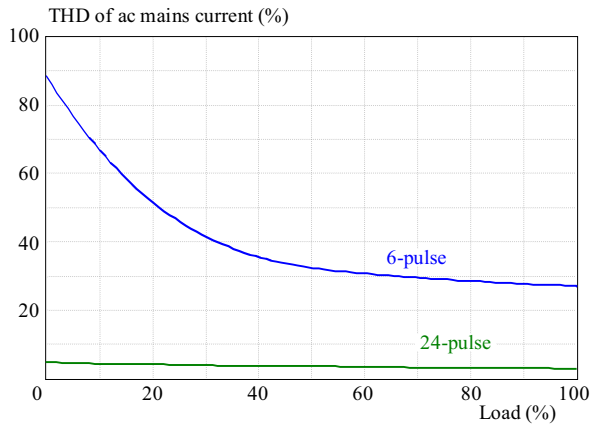
Fig. 11. Variation of THD with load on DTCIMD in 6-pulse, 12-pulse and 24-pulse ac-dc converter
