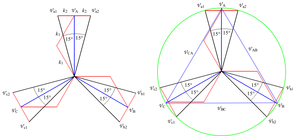
Fig. 2. Polygon connection of proposed autotransformer for 12-pulse converter and its phasor representation
