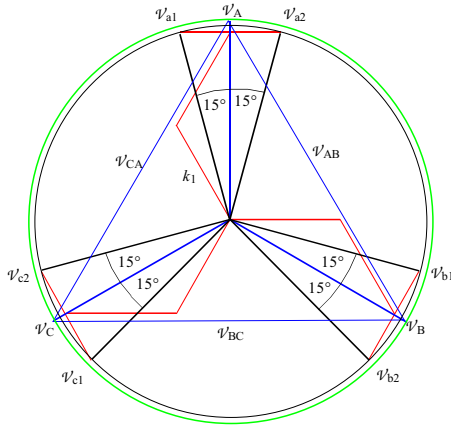
Fig. 4. Phasor diagram of voltages in the proposed autotransformer connection along with the modifications for retrofit arrangement
