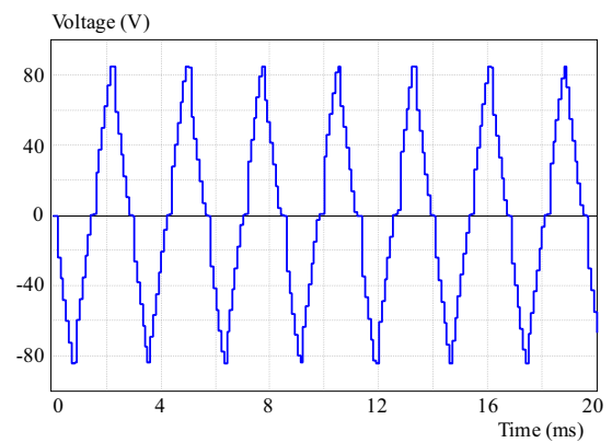
Fig. 7. Voltage waveform across the double-tap IPR
